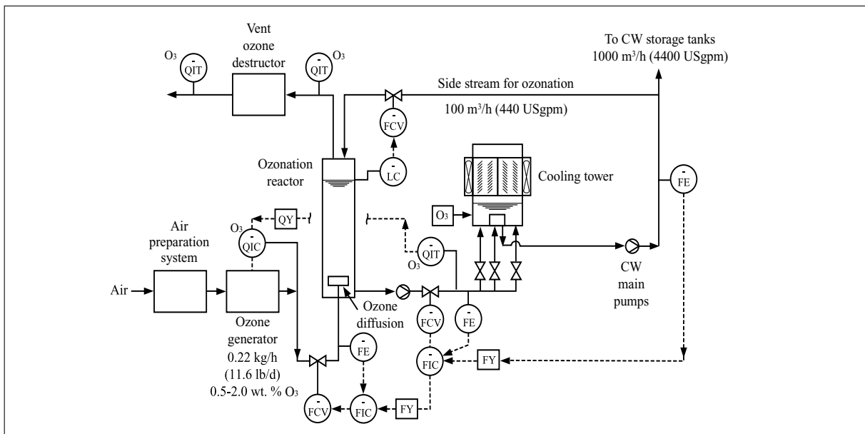
Figure 2: Ozonation system
